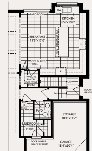
PARTIAL GROUND
