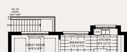
PARTIAL GROUND
