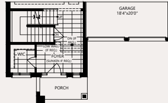
PARTIAL GROUND
