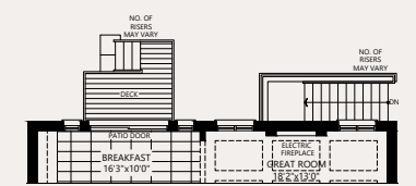
PARTIAL GROUND
