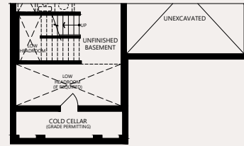
PARTIAL GROUND
