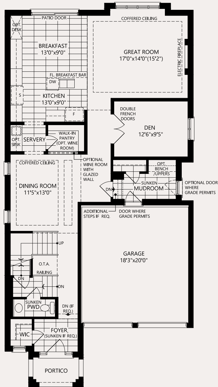
MAIN FLOOR
