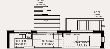
PARTIAL GROUND
