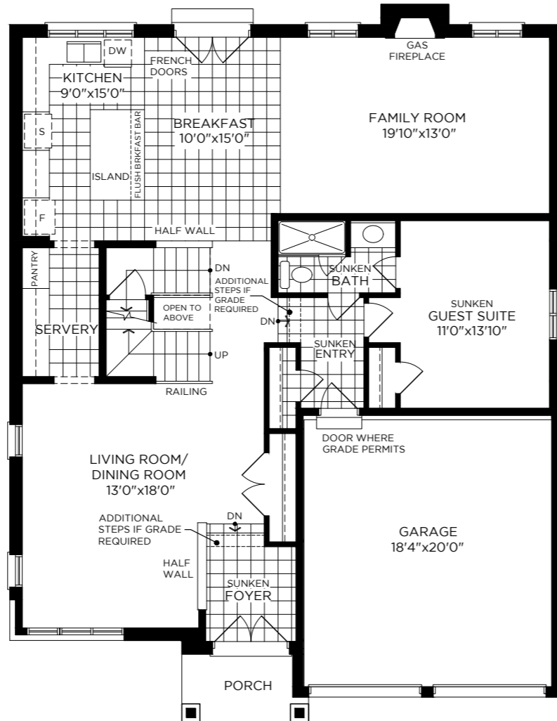
MAIN FLOOR ELEVATION A
