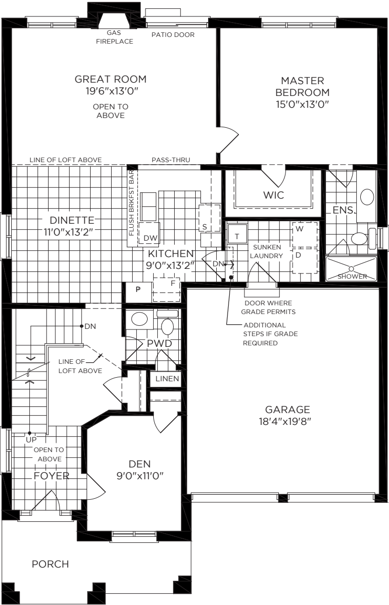
MAIN FLOOR ELEVATION B
