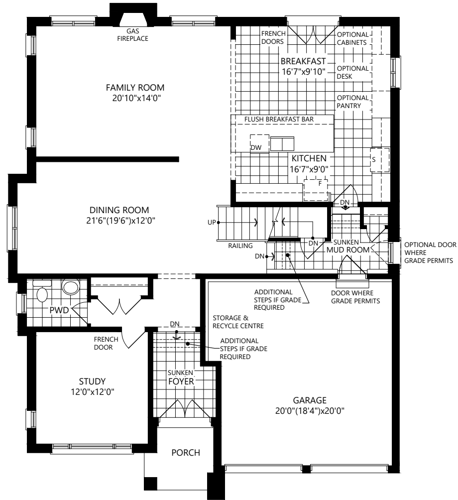
MAIN FLOOR ELEVATION A
