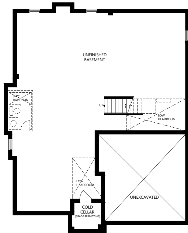
BASEMENT ELEVATION B
