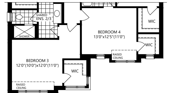
PARTIAL SECOND FLOOR ELEVATION D
