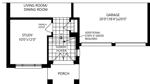
PARTIAL MAIN FLOOR ELEVATION D
