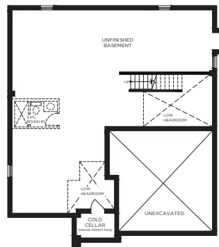
BASEMENT ELEVATION A
