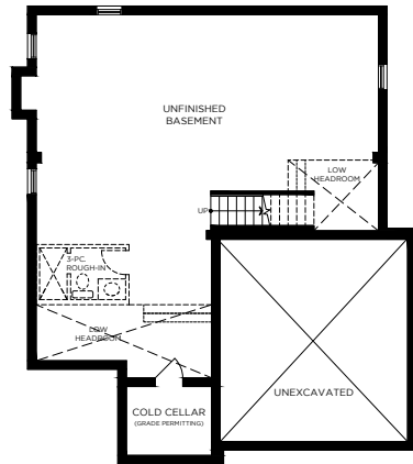
BASEMENT ELEVATION B
